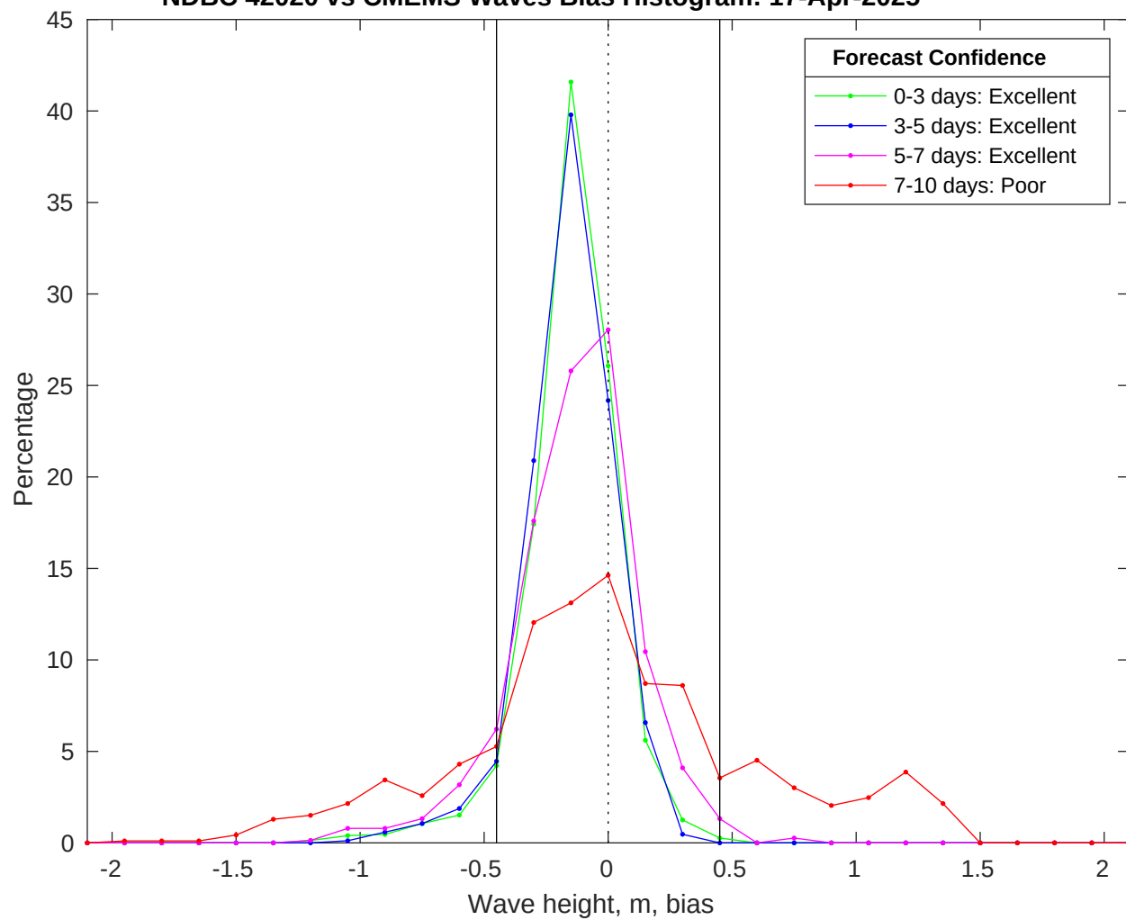
NDBC 42020 vs CMEMS Waves Bias Histogram: 17-Apr-2025
