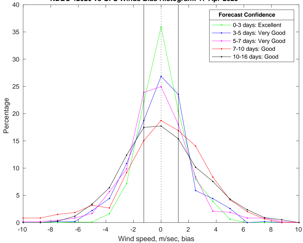
NDBC 42020 vs GFS Winds Bias Histogram: 17-Apr-2025
