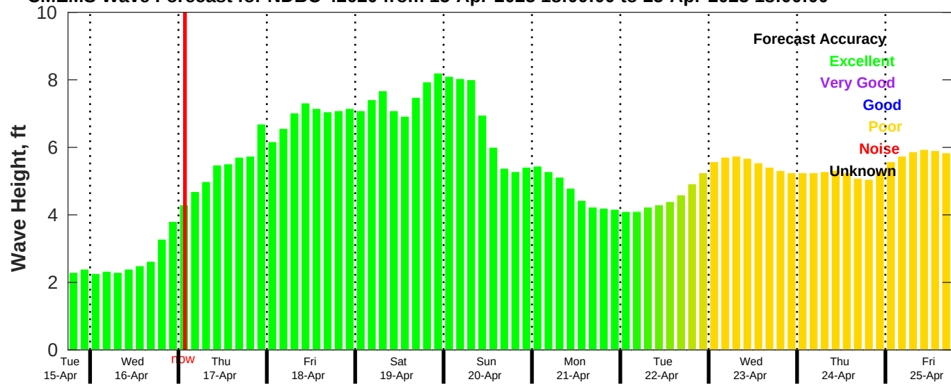
CMEMS Wave Forecast for NDBC 42020 from 15-Apr-2025 18:00:00 to 25-Apr-2025 18:00:00
