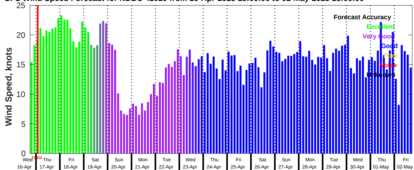
GFS Wind Speed Forecast for NDBC 42020 from 16-Apr-2025 18:00:00 to 02-May-2025 18:00:00
