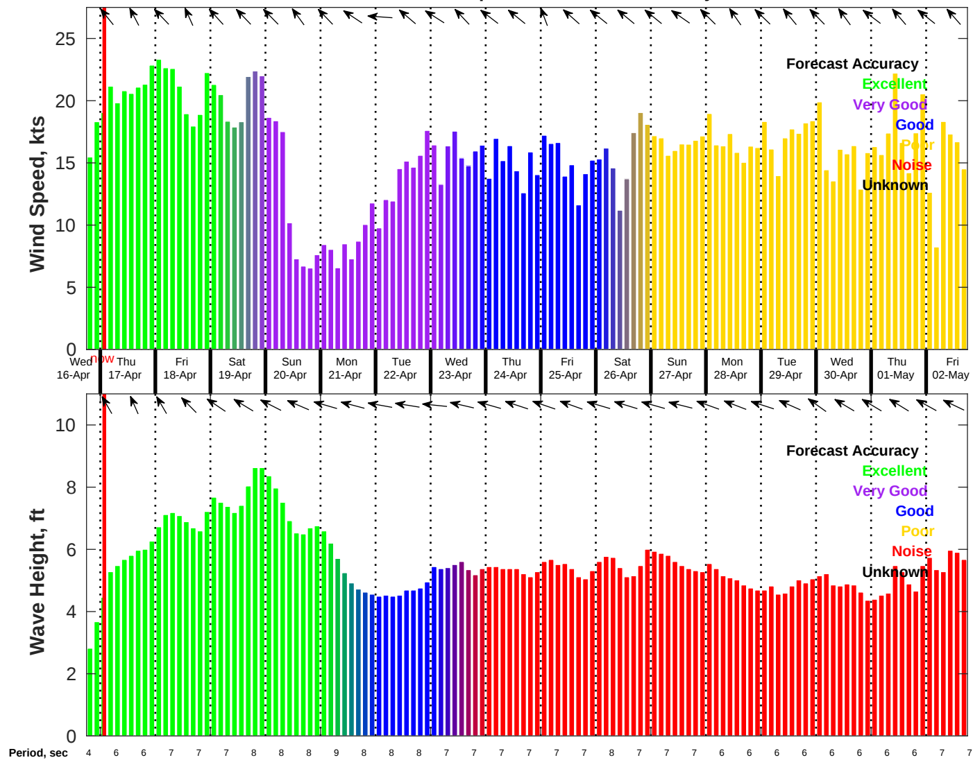
Wind & Wave Forecast for NDBC 42020 from 16-Apr-2025 18:00:00 to 02-May-2025 18:00:00
