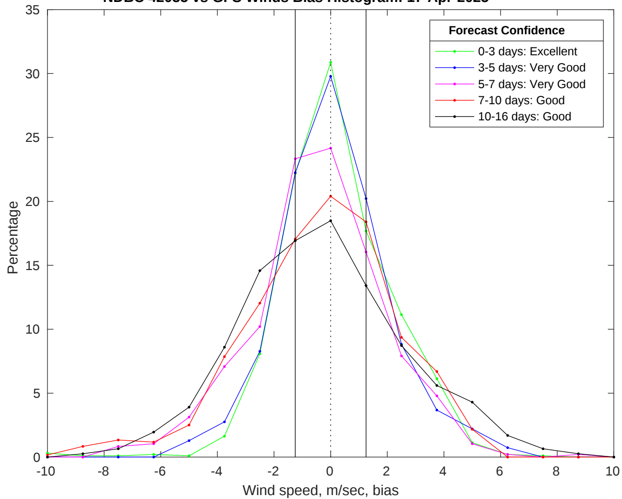
NDBC 42035 vs GFS Winds Bias Histogram: 17-Apr-2025
