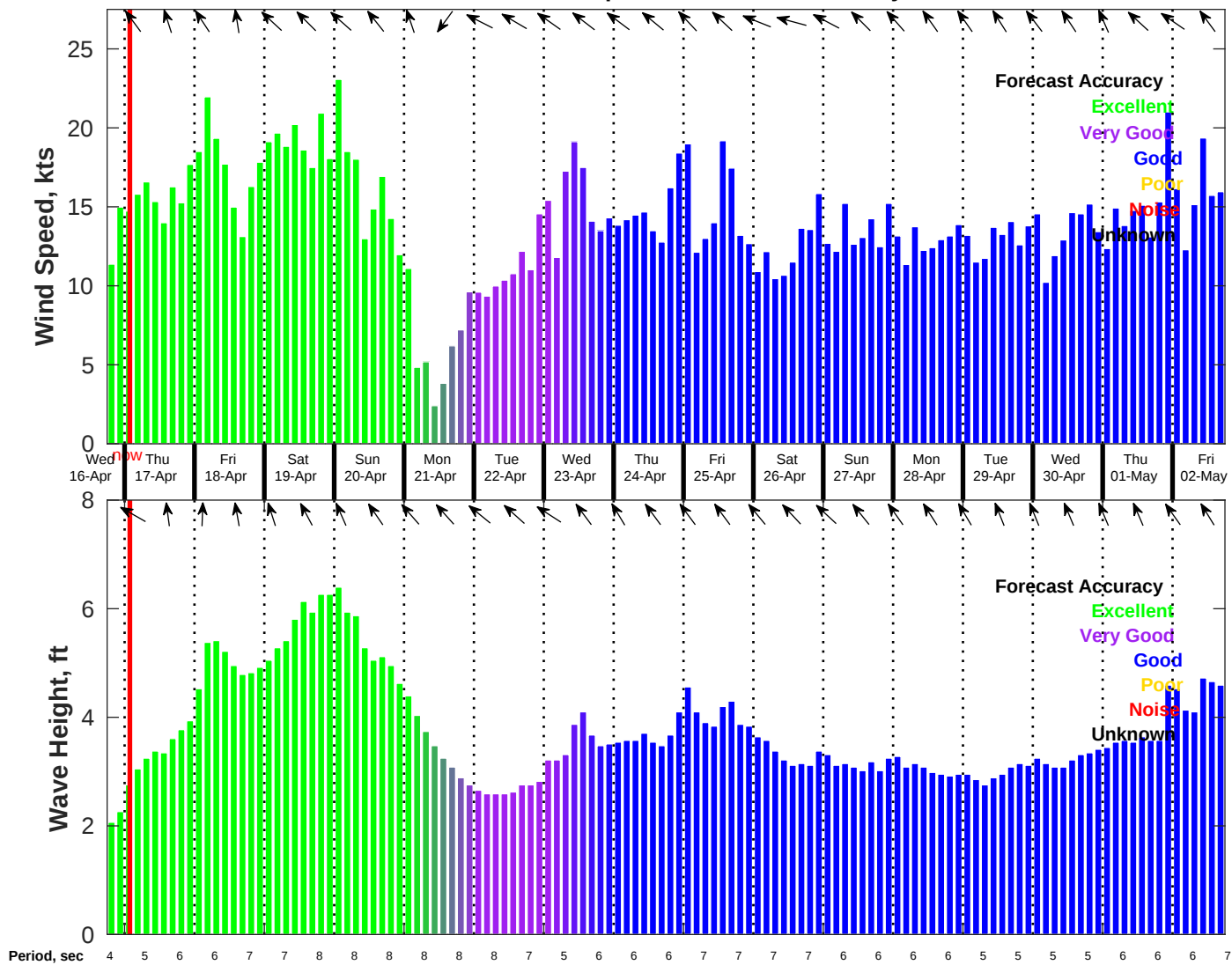
Wind & Wave Forecast for NDBC 42035 from 16-Apr-2025 18:00:00 to 02-May-2025 18:00:00
