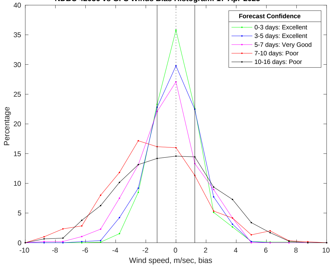
NDBC 42036 vs GFS Winds Bias Histogram: 17-Apr-2025
