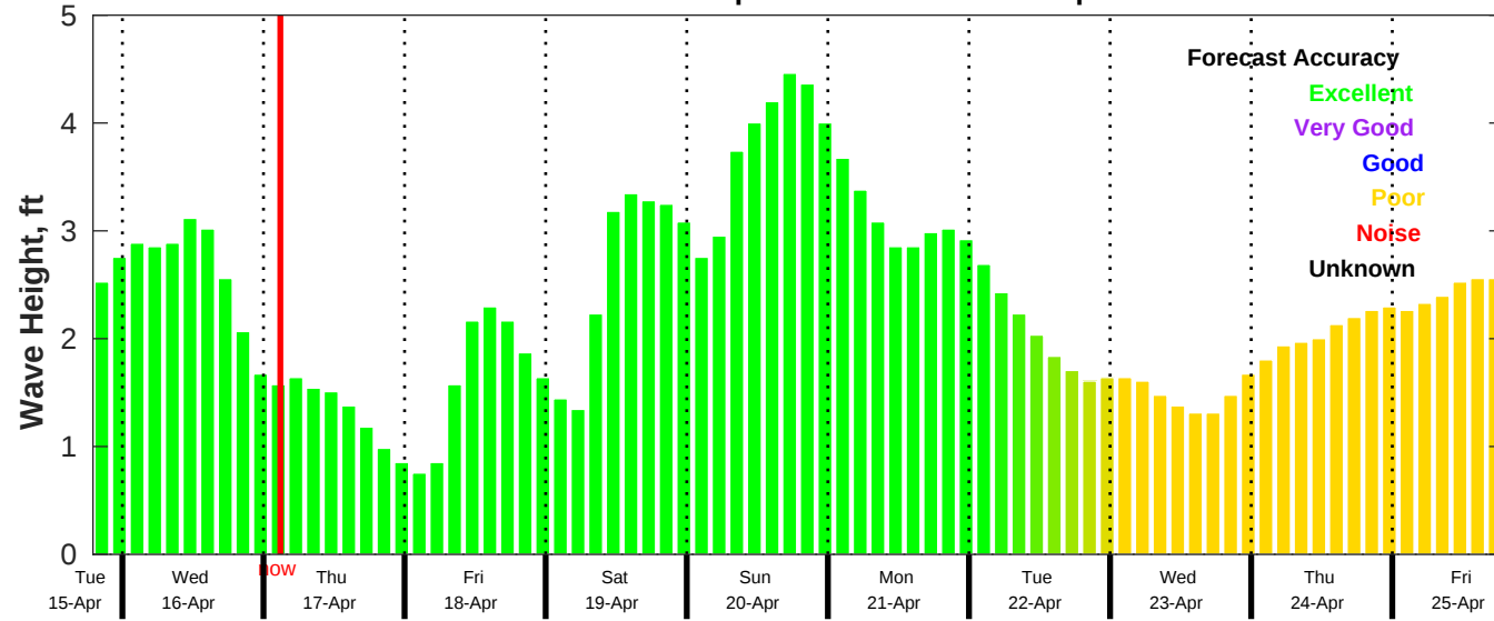
CMEMS Wave Forecast for NDBC 42036 from 15-Apr-2025 19:00:00 to 25-Apr-2025 19:00:00
