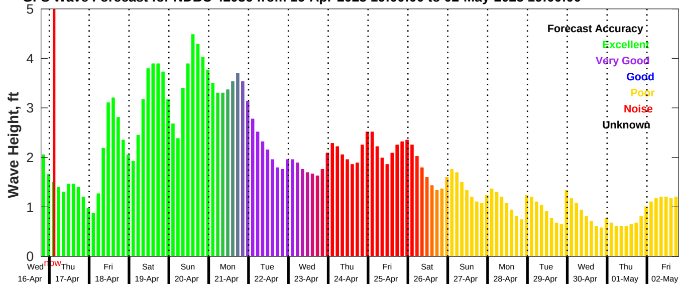
GFS Wave Forecast for NDBC 42036 from 16-Apr-2025 19:00:00 to 02-May-2025 19:00:00
