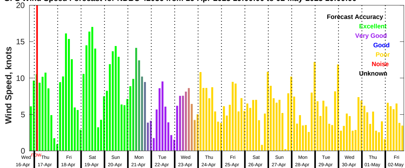
GFS Wind Speed Forecast for NDBC 42036 from 16-Apr-2025 19:00:00 to 02-May-2025 19:00:00
