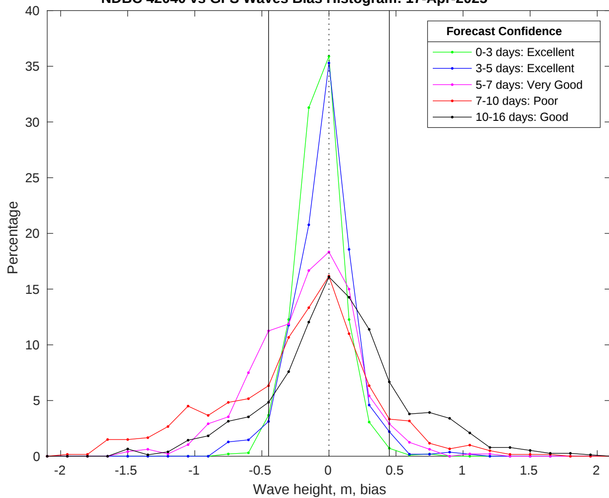
NDBC 42040 vs GFS Waves Bias Histogram: 17-Apr-2025
