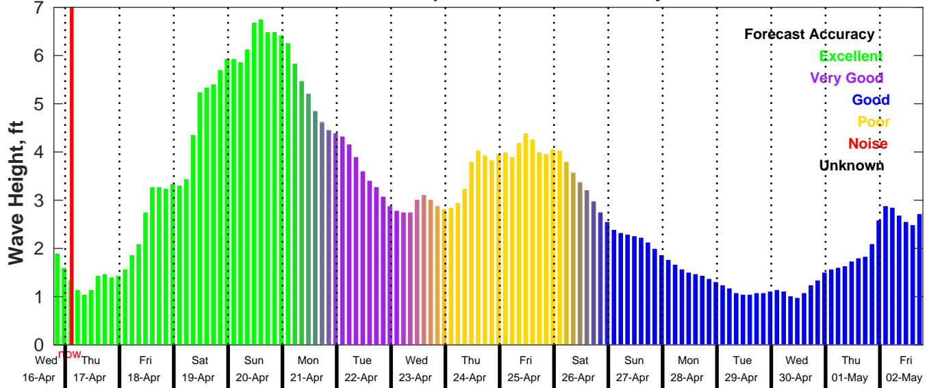
GFS Wave Forecast for NDBC 42040 from 16-Apr-2025 19:00:00 to 02-May-2025 19:00:00
