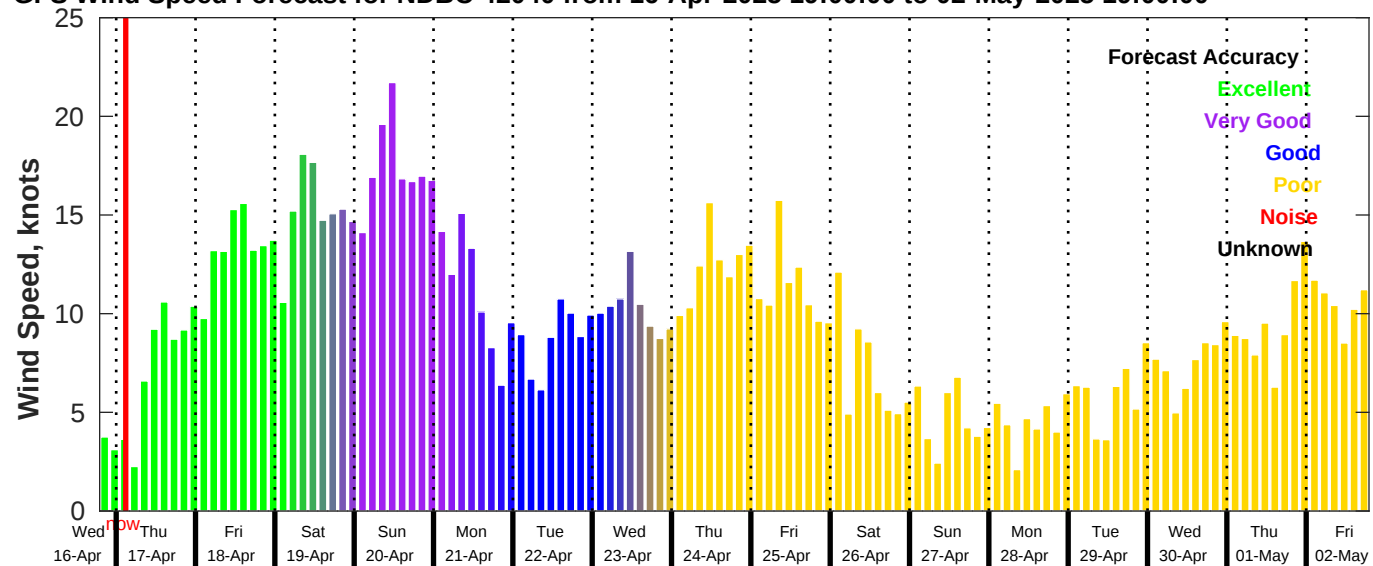
GFS Wind Speed Forecast for NDBC 42040 from 16-Apr-2025 19:00:00 to 02-May-2025 19:00:00
