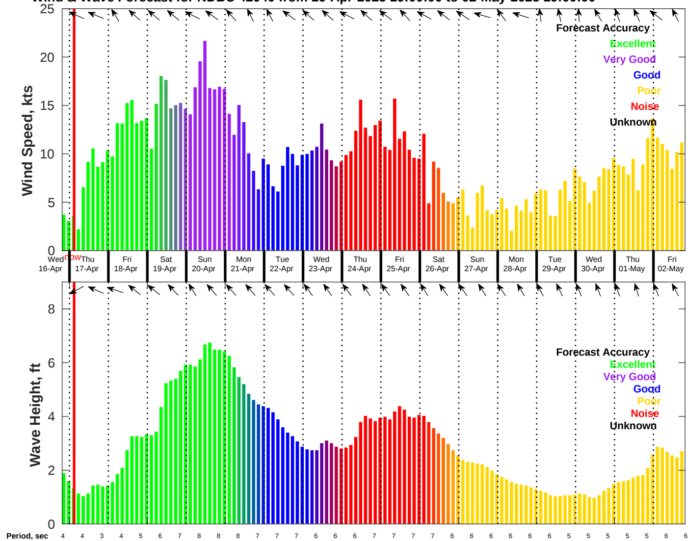
Wind & Wave Forecast for NDBC 42040 from 16-Apr-2025 19:00:00 to 02-May-2025 19:00:00
