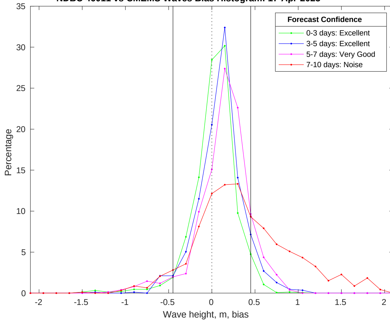
NDBC 46011 vs CMEMS Waves Bias Histogram: 17-Apr-2025
