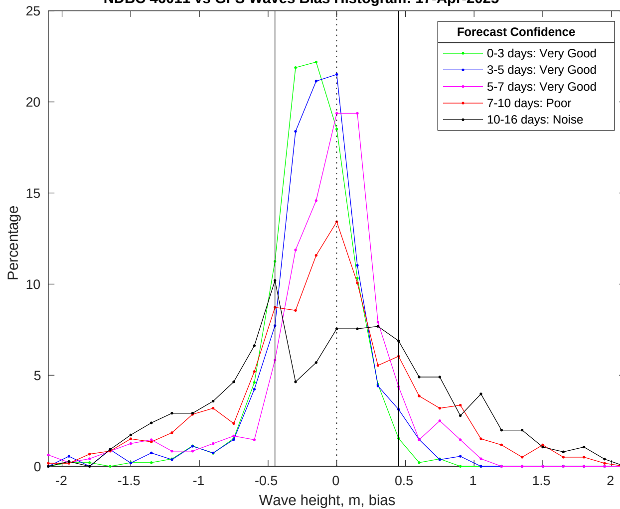
NDBC 46011 vs GFS Waves Bias Histogram: 17-Apr-2025
