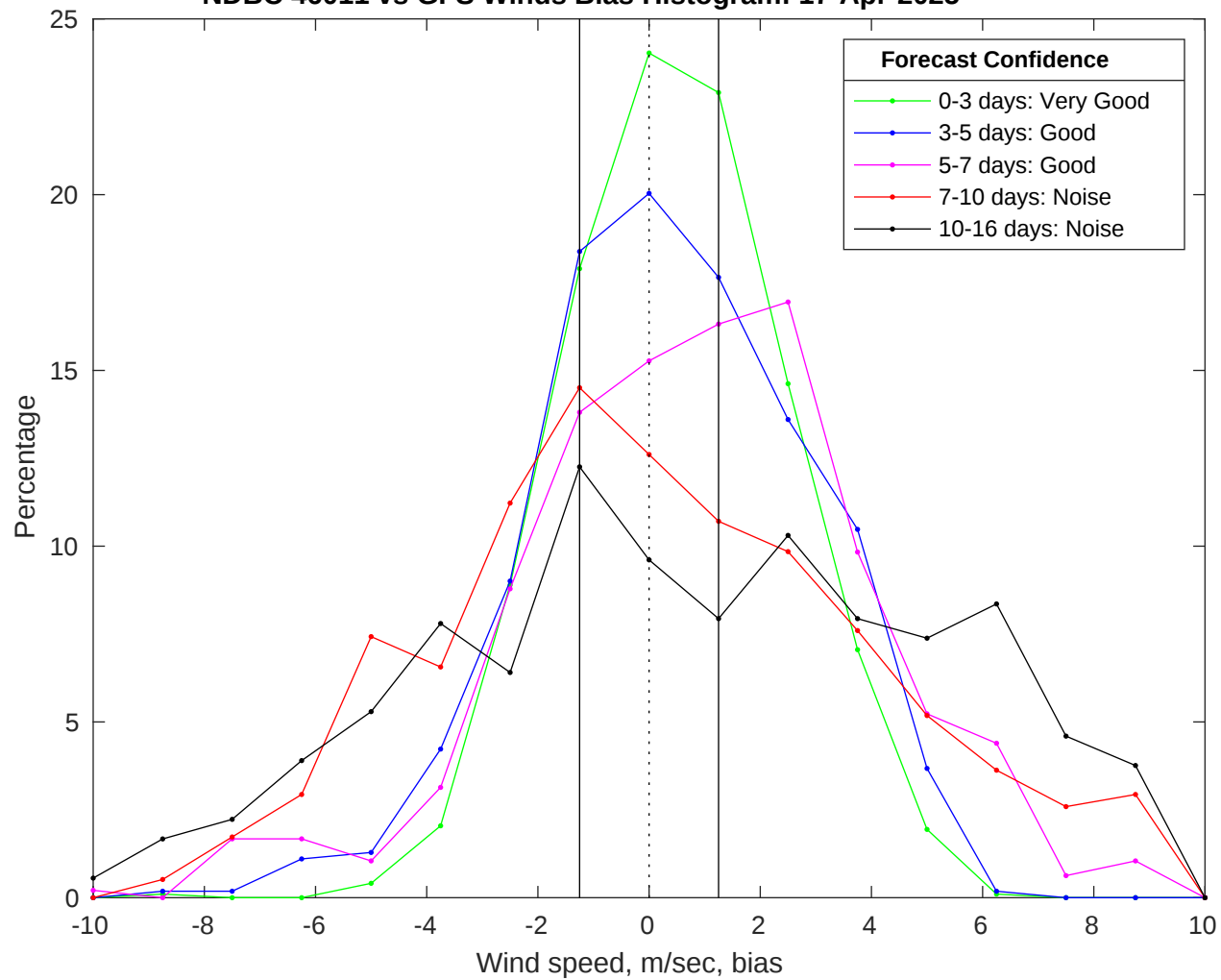
NDBC 46011 vs GFS Winds Bias Histogram: 17-Apr-2025
