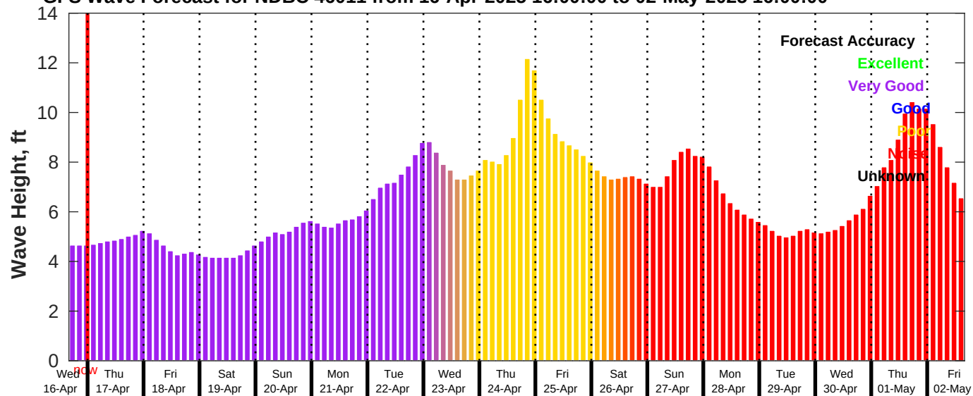
GFS Wave Forecast for NDBC 46011 from 16-Apr-2025 16:00:00 to 02-May-2025 16:00:00
