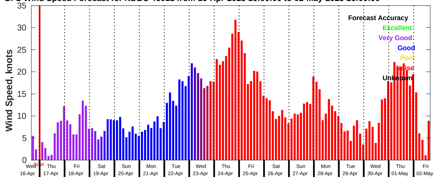
GFS Wind Speed Forecast for NDBC 46011 from 16-Apr-2025 16:00:00 to 02-May-2025 16:00:00
