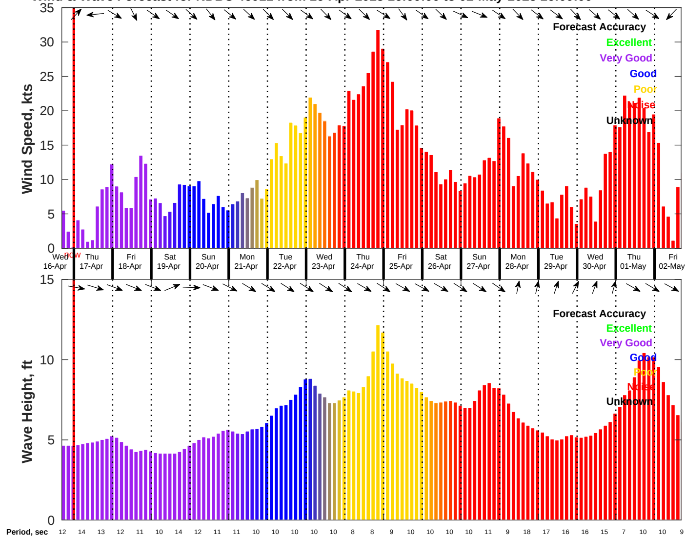
Wind & Wave Forecast for NDBC 46011 from 16-Apr-2025 16:00:00 to 02-May-2025 16:00:00
