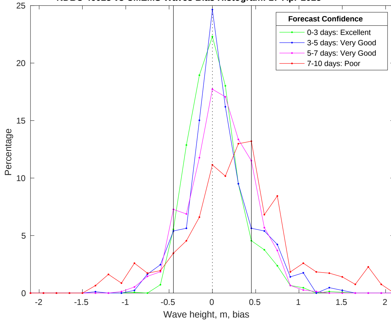
NDBC 46028 vs CMEMS Waves Bias Histogram: 17-Apr-2025
