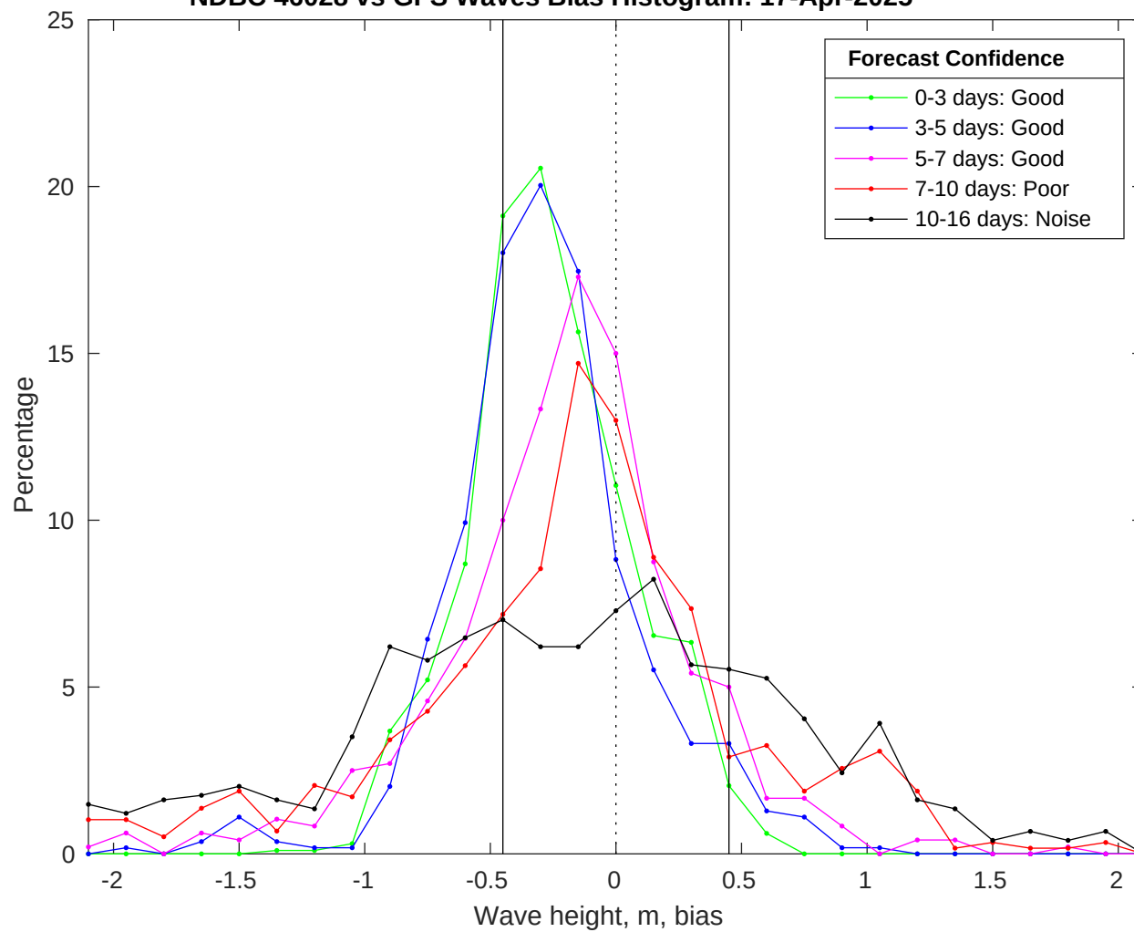
NDBC 46028 vs GFS Waves Bias Histogram: 17-Apr-2025
