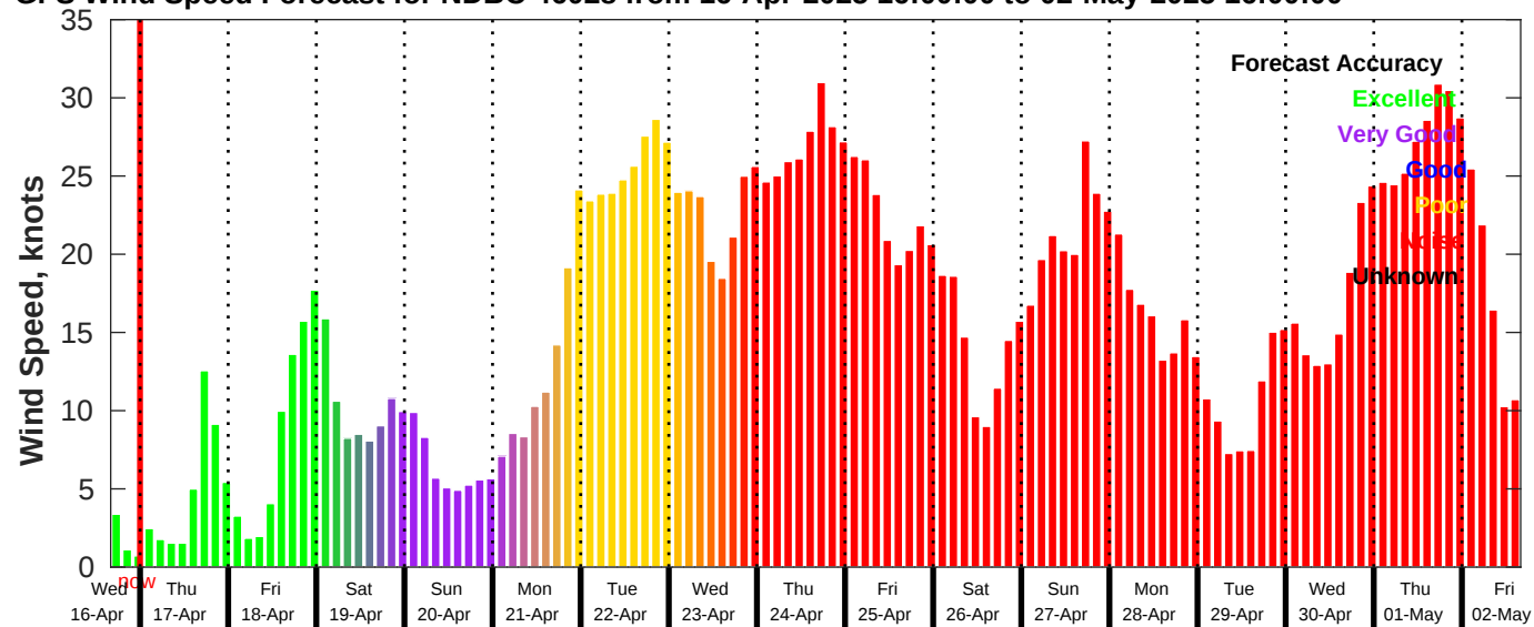
GFS Wind Speed Forecast for NDBC 46028 from 16-Apr-2025 16:00:00 to 02-May-2025 16:00:00
