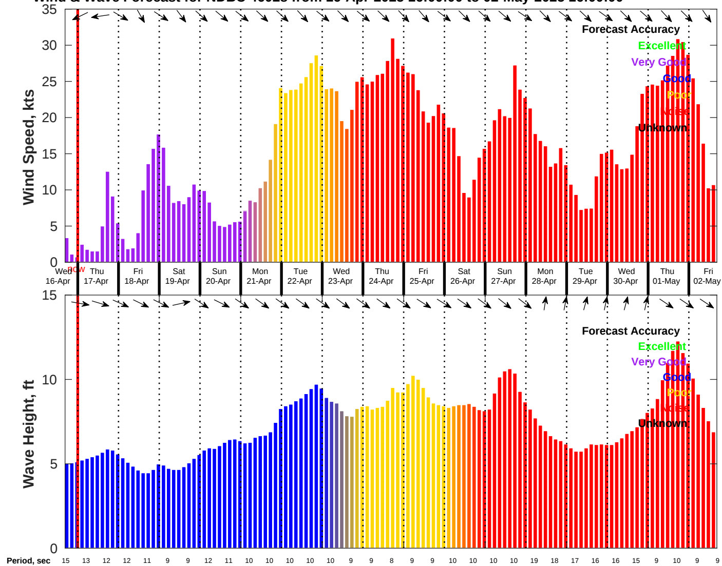
Wind & Wave Forecast for NDBC 46028 from 16-Apr-2025 16:00:00 to 02-May-2025 16:00:00
