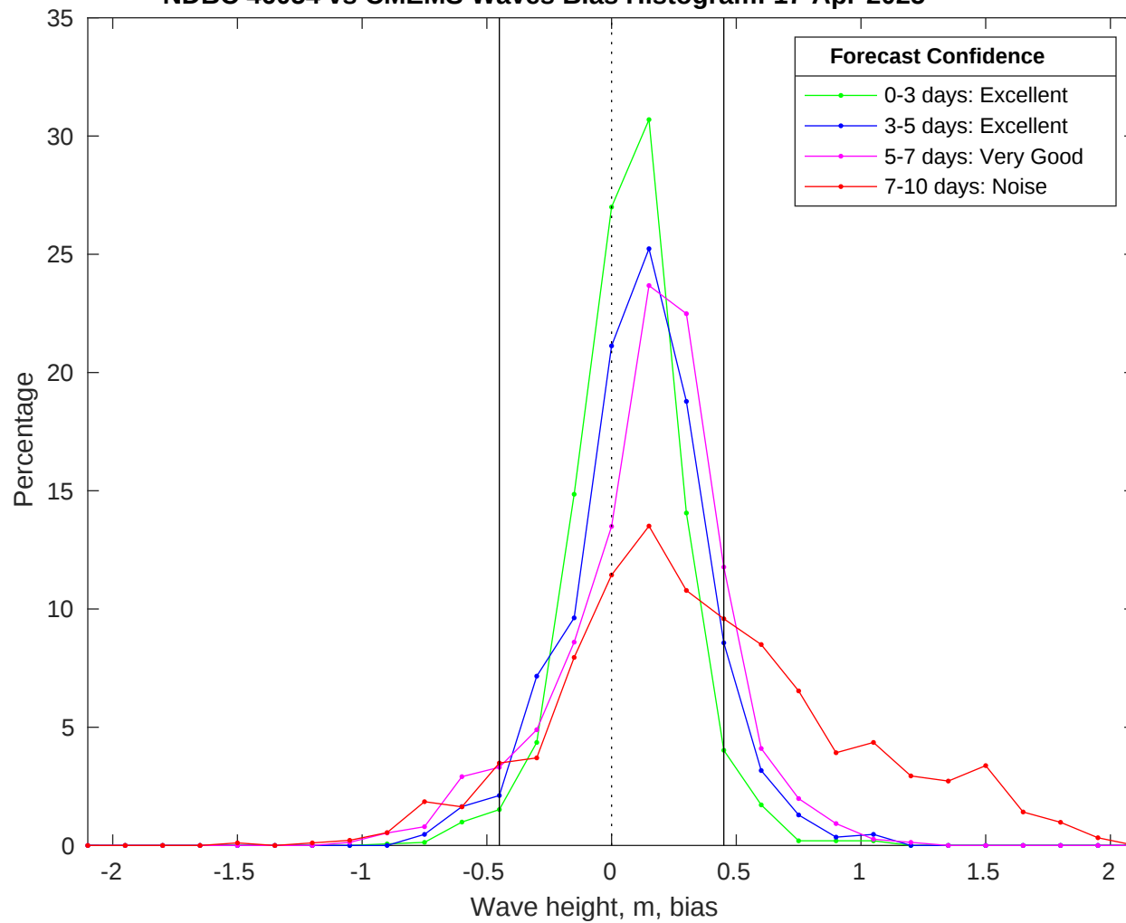
NDBC 46054 vs CMEMS Waves Bias Histogram: 17-Apr-2025
