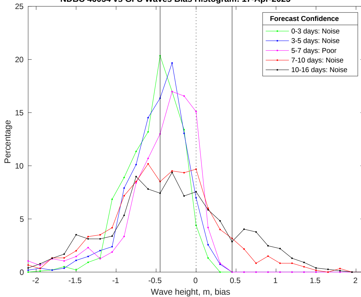
NDBC 46054 vs GFS Waves Bias Histogram: 17-Apr-2025
