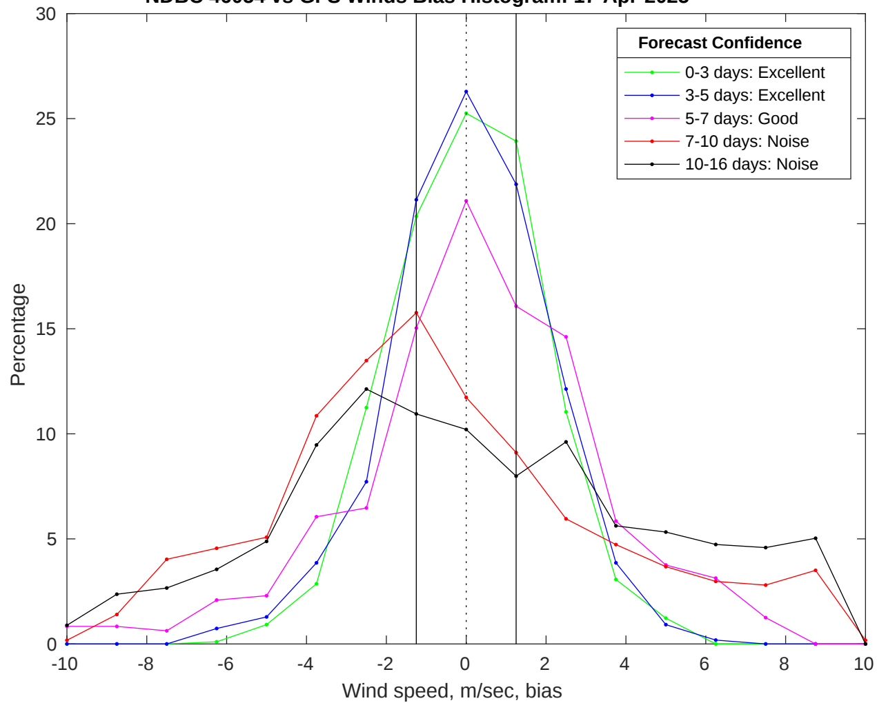
NDBC 46054 vs GFS Winds Bias Histogram: 17-Apr-2025
