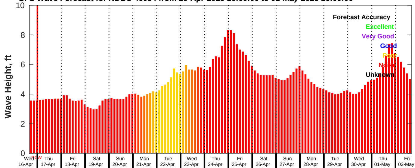
GFS Wave Forecast for NDBC 46054 from 16-Apr-2025 16:00:00 to 02-May-2025 16:00:00
