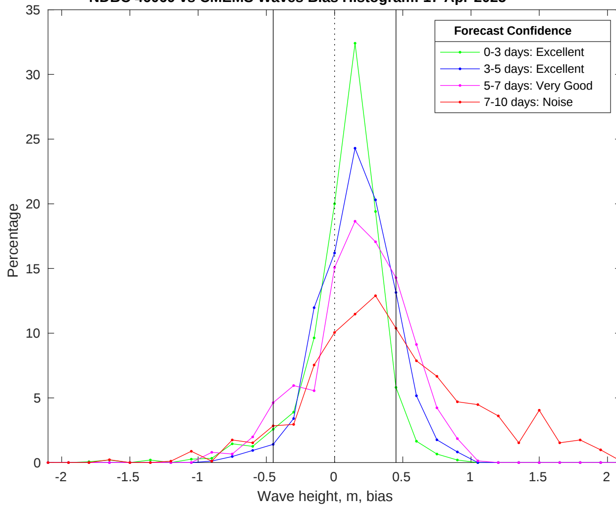
NDBC 46069 vs CMEMS Waves Bias Histogram: 17-Apr-2025
