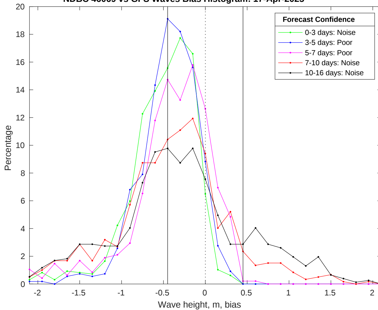
NDBC 46069 vs GFS Waves Bias Histogram: 17-Apr-2025
