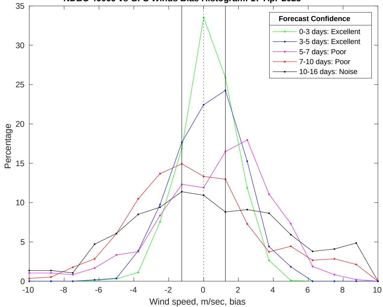
NDBC 46069 vs GFS Winds Bias Histogram: 17-Apr-2025
