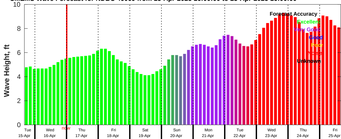
CMEMS Wave Forecast for NDBC 46069 from 15-Apr-2025 16:00:00 to 25-Apr-2025 16:00:00
