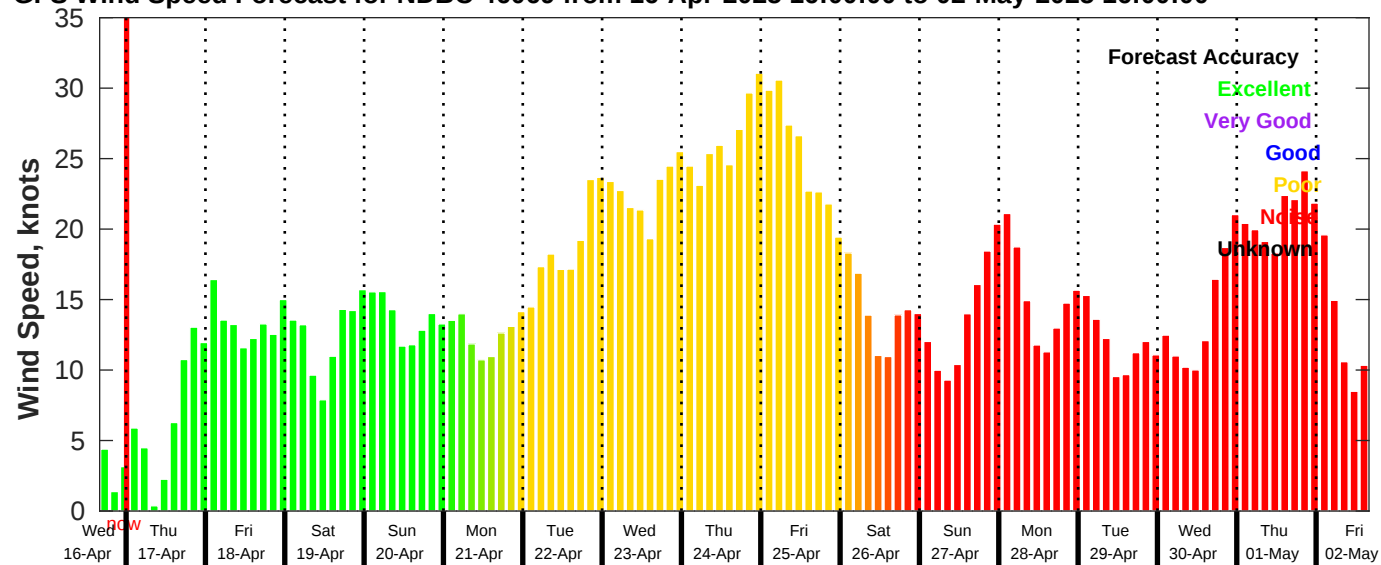
GFS Wind Speed Forecast for NDBC 46069 from 16-Apr-2025 16:00:00 to 02-May-2025 16:00:00
