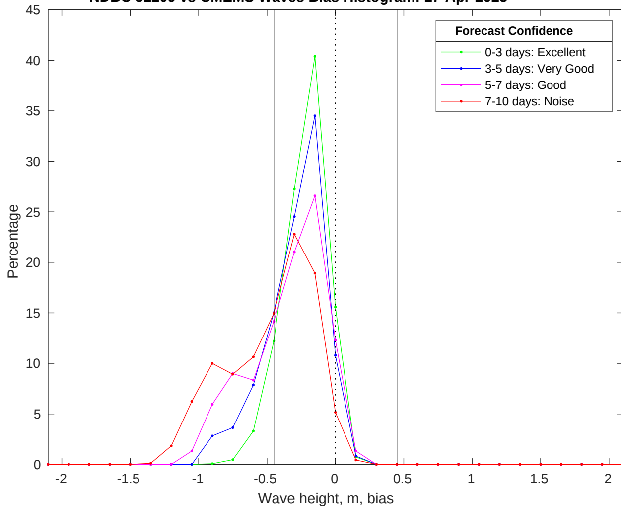
NDBC 51209 vs CMEMS Waves Bias Histogram: 17-Apr-2025
