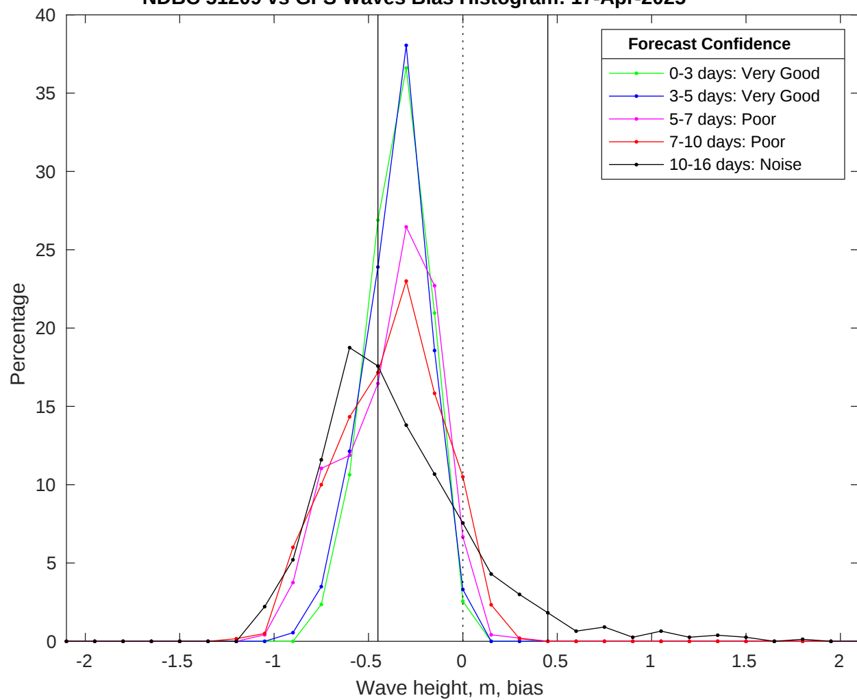
NDBC 51209 vs GFS Waves Bias Histogram: 17-Apr-2025
