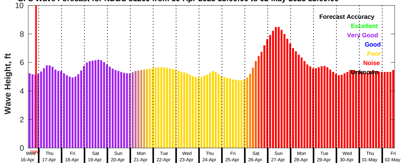
GFS Wave Forecast for NDBC 51209 from 16-Apr-2025 13:00:00 to 02-May-2025 13:00:00
