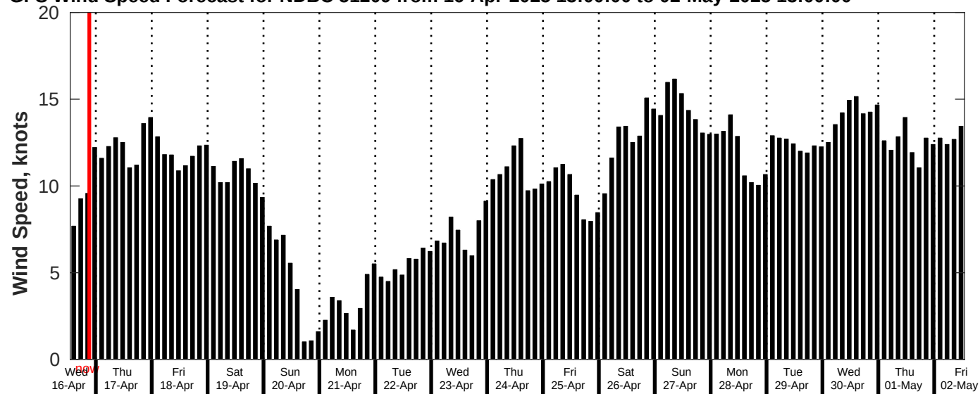
GFS Wind Speed Forecast for NDBC 51209 from 16-Apr-2025 13:00:00 to 02-May-2025 13:00:00
