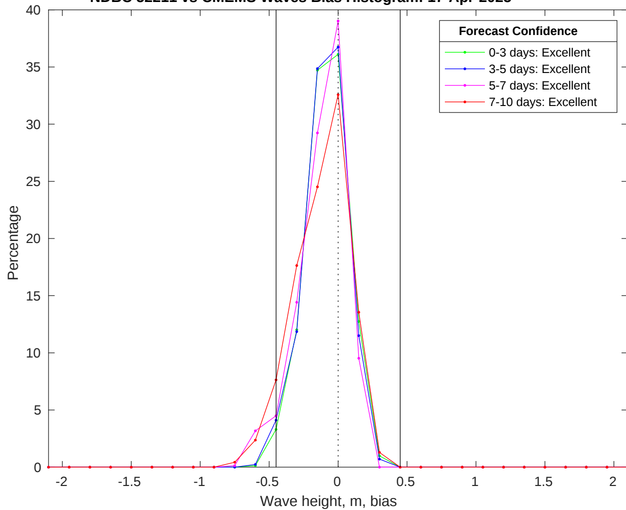
NDBC 52211 vs CMEMS Waves Bias Histogram: 17-Apr-2025
