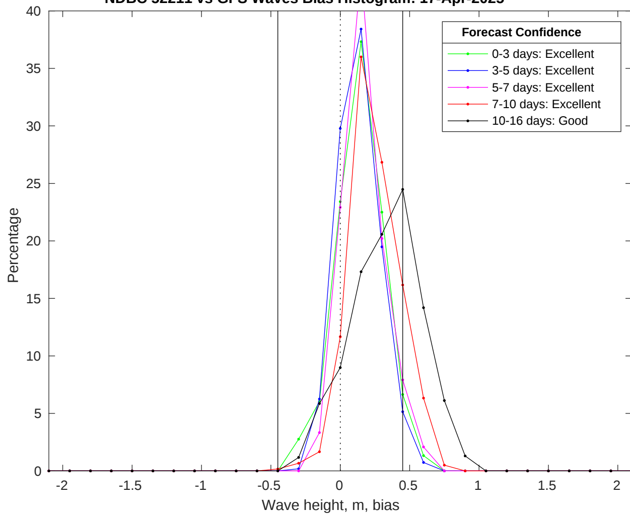
NDBC 52211 vs GFS Waves Bias Histogram: 17-Apr-2025
