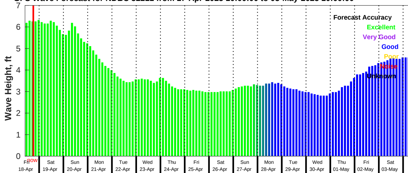
GFS Wave Forecast for NDBC 52211 from 17-Apr-2025 10:00:00 to 03-May-2025 10:00:00
