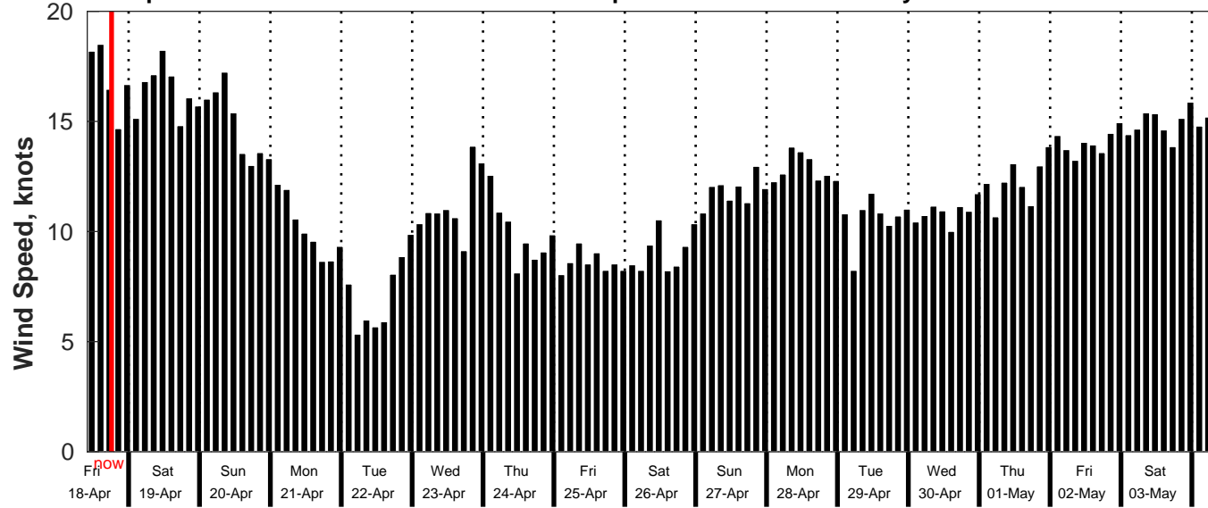
GFS Wind Speed Forecast for NDBC 52211 from 17-Apr-2025 10:00:00 to 03-May-2025 10:00:00
