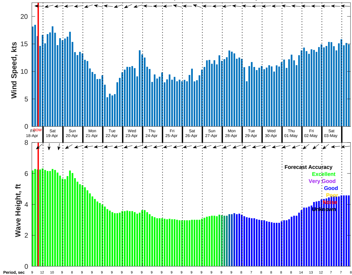
Wind & Wave Forecast for NDBC 52211 from 17-Apr-2025 10:00:00 to 03-May-2025 10:00:00
