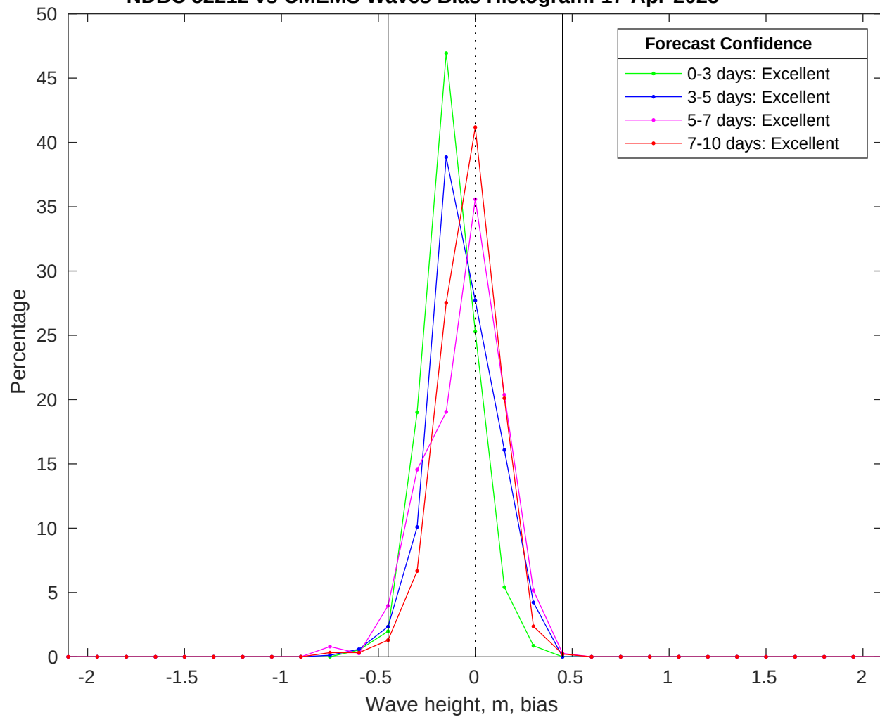
NDBC 52212 vs CMEMS Waves Bias Histogram: 17-Apr-2025
