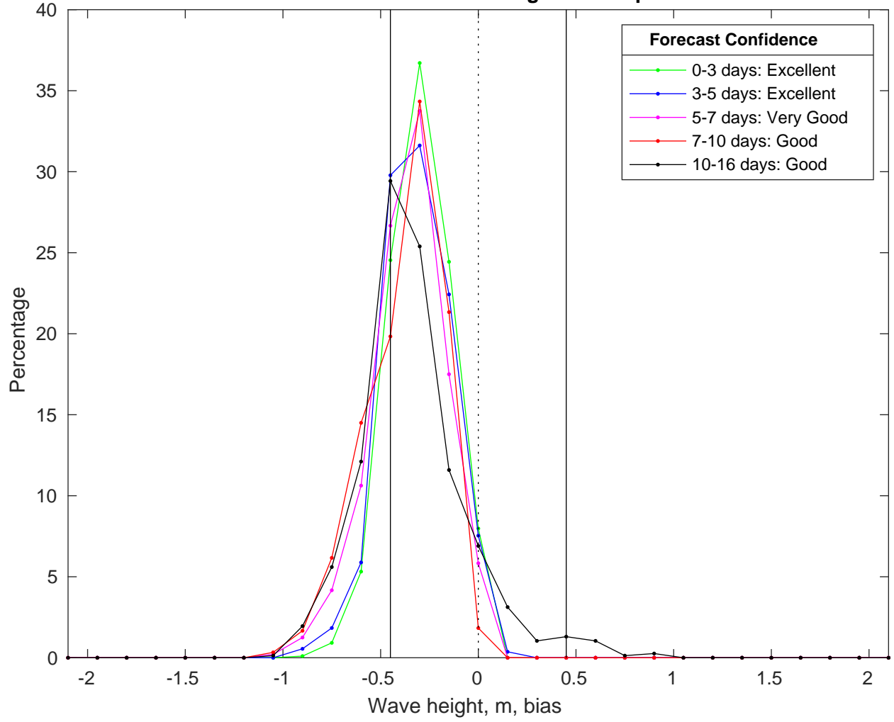
NDBC 52212 vs GFS Waves Bias Histogram: 17-Apr-2025
