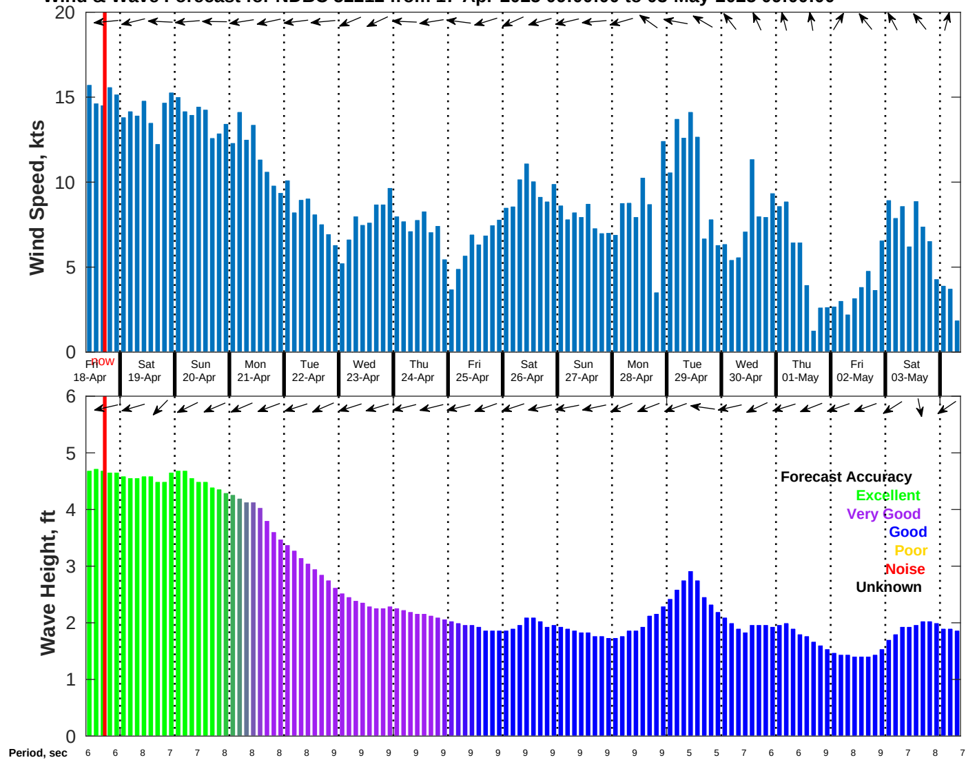
Wind & Wave Forecast for NDBC 52212 from 17-Apr-2025 09:00:00 to 03-May-2025 09:00:00
