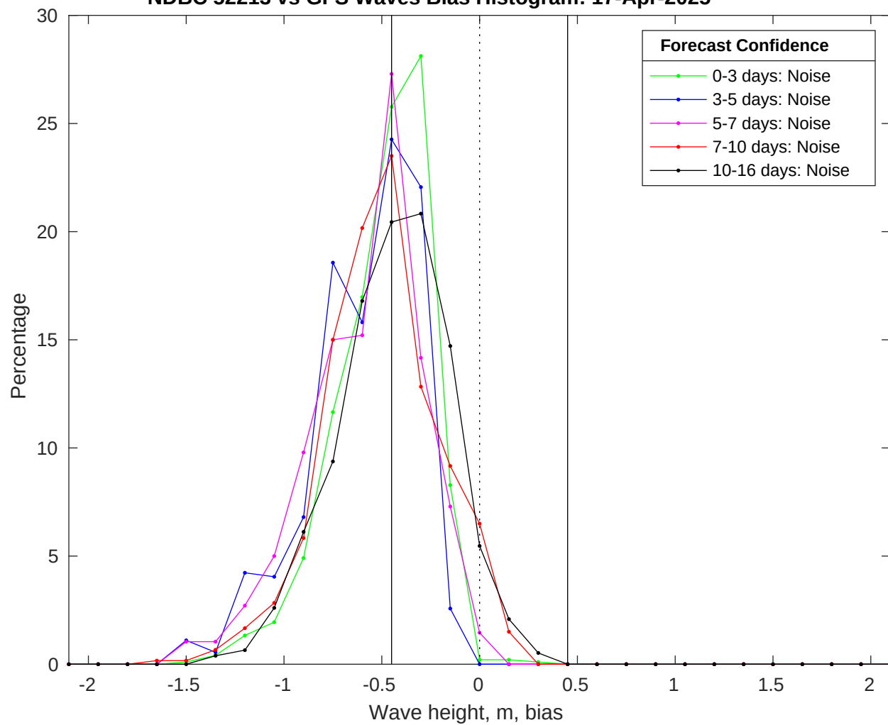
NDBC 52213 vs GFS Waves Bias Histogram: 17-Apr-2025
