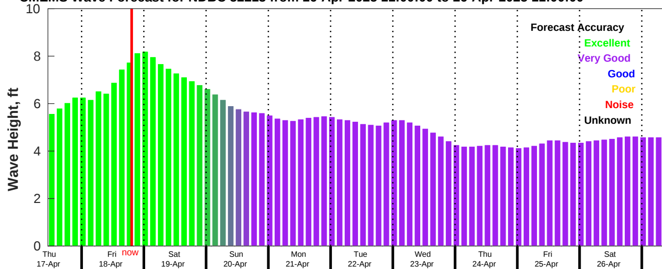
CMEMS Wave Forecast for NDBC 52213 from 16-Apr-2025 11:00:00 to 26-Apr-2025 11:00:00
