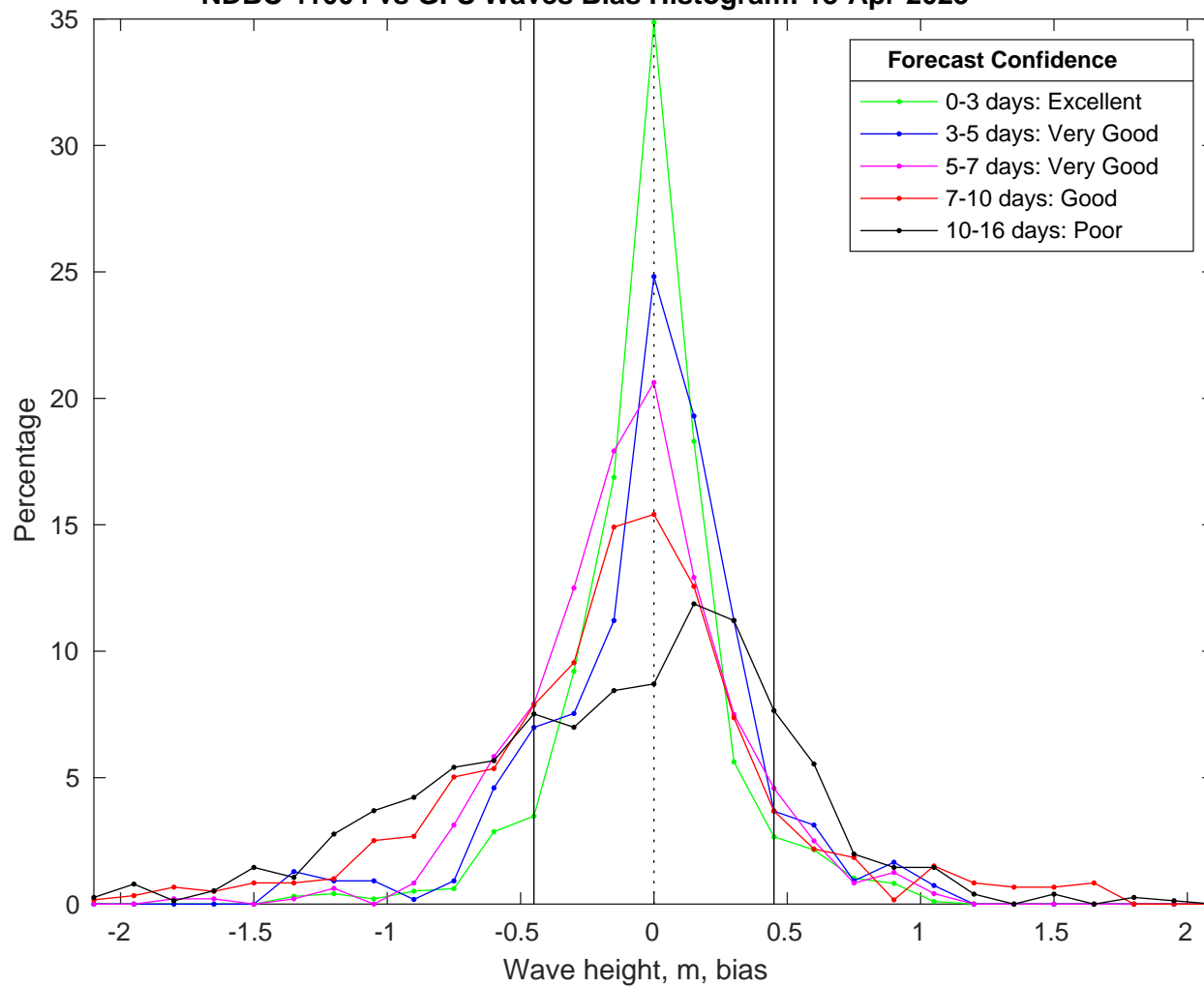
NDBC 41004 vs GFS Waves Bias Histogram: 18-Apr-2025
