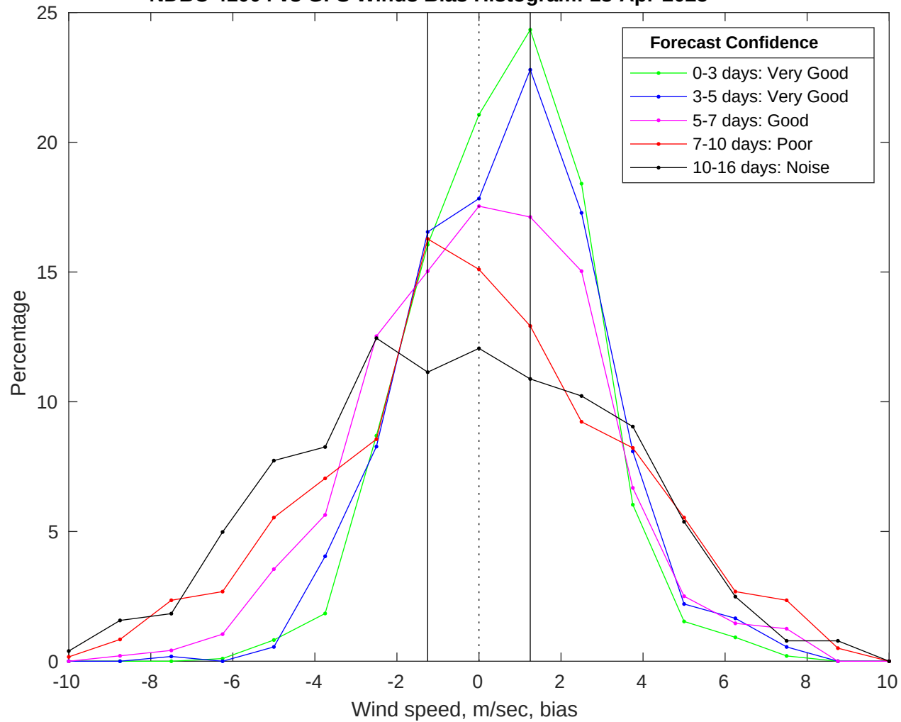
NDBC 41004 vs GFS Winds Bias Histogram: 18-Apr-2025
